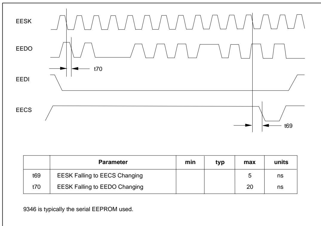
Figure 12.16 - EEPROM Write
