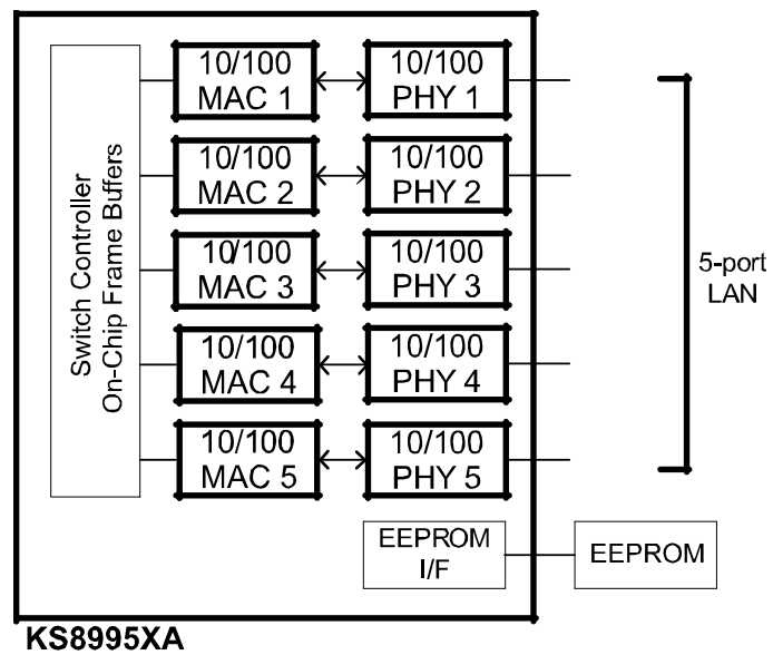
Figure 3. Standalone Switch
