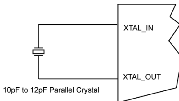
Figure 7. Crystal Input Interface
