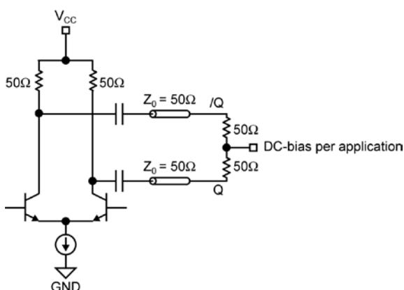
Figure 4c. CML AC-Coupled Termination
