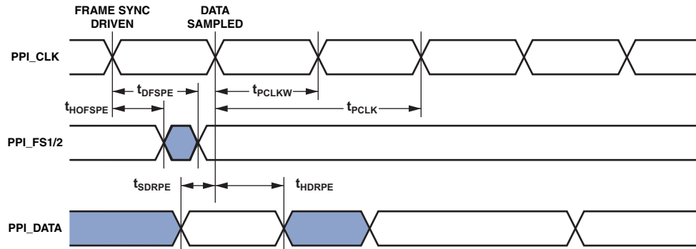
Figure 20. PPI GP Rx Mode with Internal Frame Sync Timing
