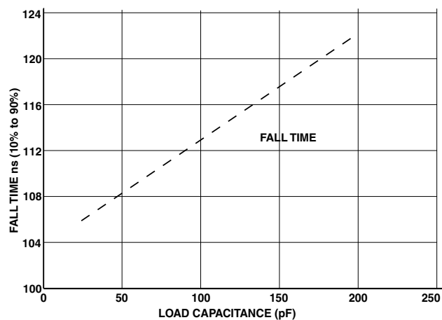
Figure 56. Typical Fall Time (10% to 90%) vs. Load Capacitance for Driver E at V_{DDEXT} = 3.65 \text{ V (Max)}
