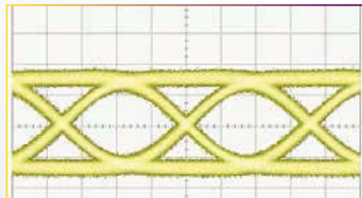
28.1 Gbps Eye Diagram for 100 GbE Applications
