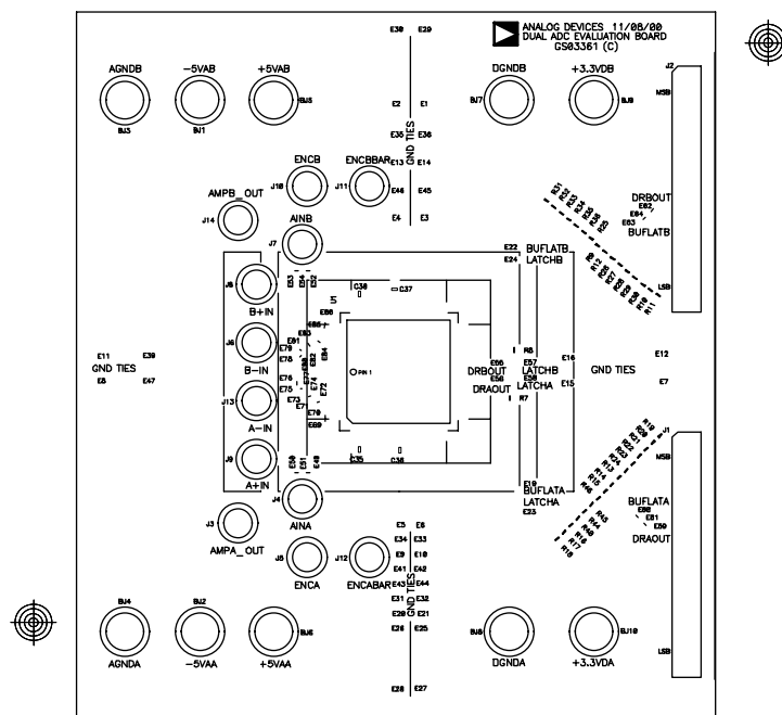
Figure 24. Top Silk
