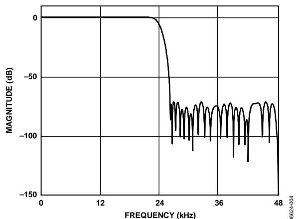
Figure 4. DAC Stop-Band Filter Response, 48 kHz
