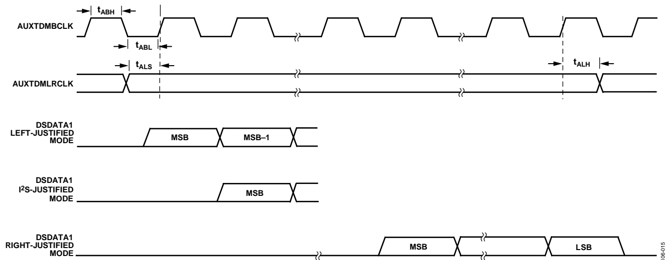
Figure 17. AXTDM Serial Timing
