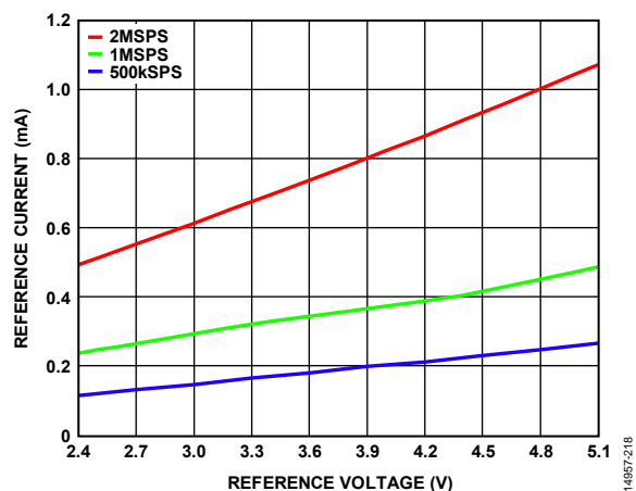
Figure 28. Reference Current vs. Reference Voltages
