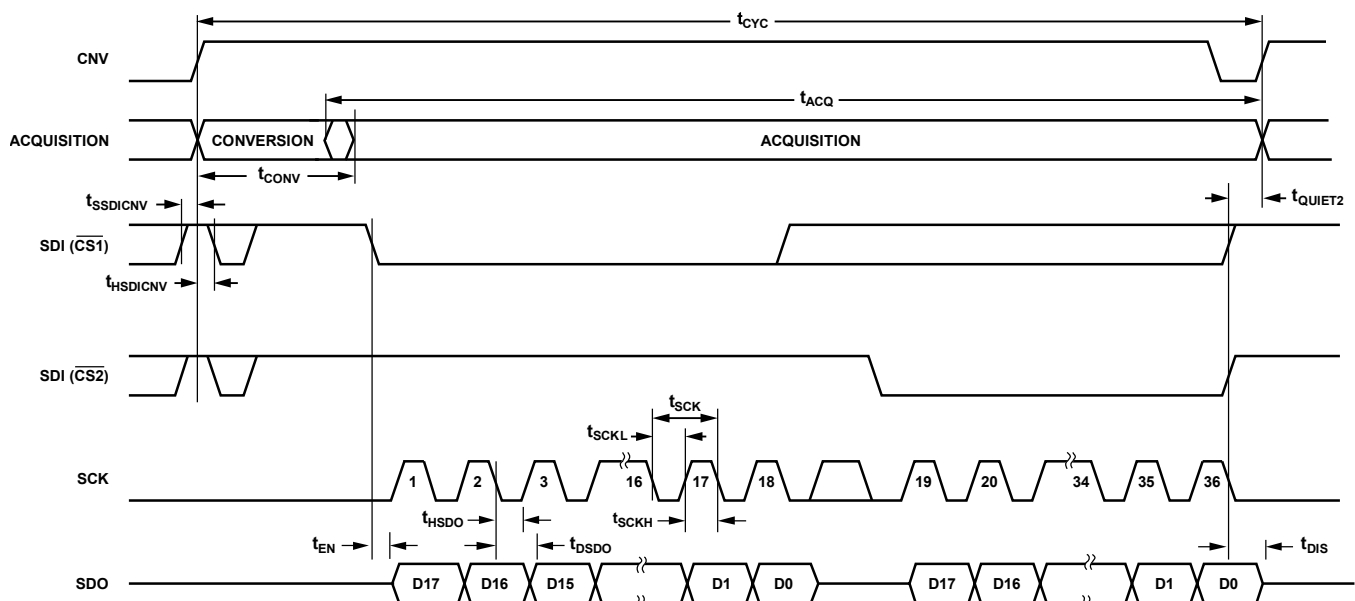
Figure 62. \overline{\text{CS}} Mode, 4-Wire Without Busy Indicator Serial Interface Timing Diagram
