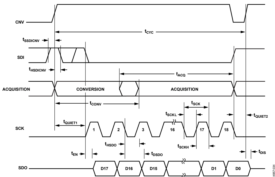
Figure 60. \overline{\text{CS}} Mode, 4-Wire Turbo Mode Timing Diagram
