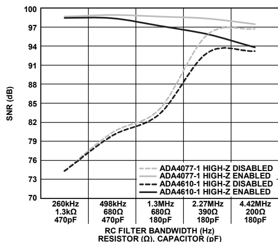
Figure 45. SNR vs. RC Filter Bandwidths for Various Precision ADC Drivers, f_{IN} = 1 kHz (Turbo Mode On, High-Z Enabled/Disabled), V_{DD} = 1.8 V, V_{IO} = 3.3 V, V_{REF} = 5 V, 25^{\circ}\text{C}
