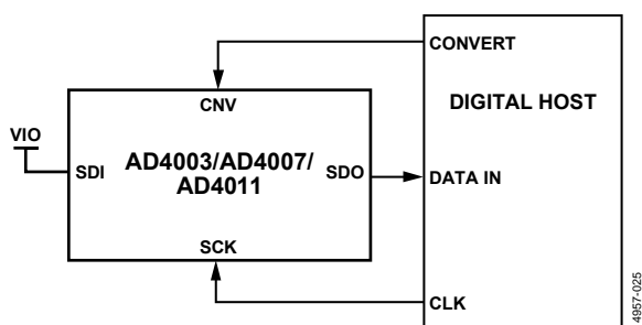
Figure 55. \overline{\text{CS}} Mode, 3-Wire Without Busy Indicator Connection Diagram (SDI High)
