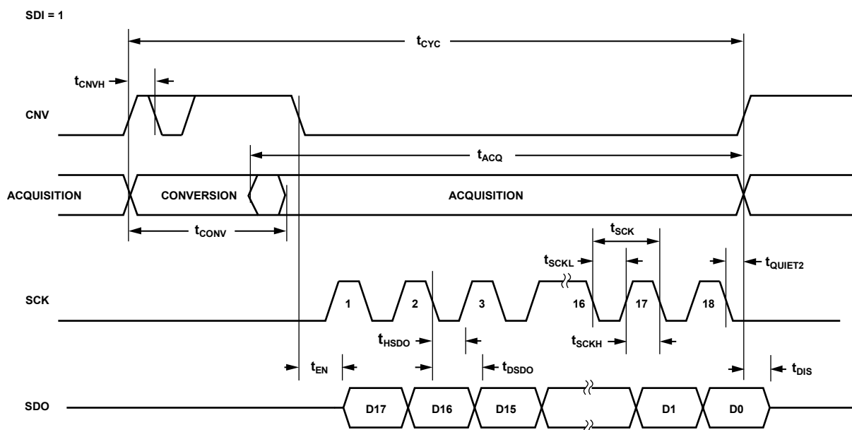
Figure 56. \overline{\text{CS}} Mode, 3-Wire Without Busy Indicator Serial Interface Timing Diagram (SDI High)
