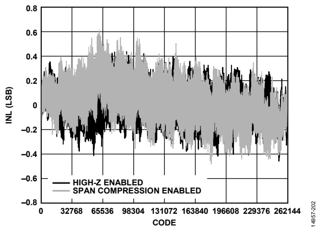
Figure 7. INL vs. Code, High-Z and Span Compression Modes Enabled, V_{REF} = 5\text{ V}
