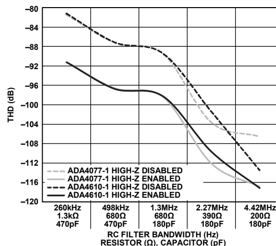
Figure 46. THD vs. RC Filter Bandwidths for Various Precision ADC Drivers, f_{IN} = 1 kHz (Turbo Mode On, High-Z Enabled/Disabled) V_{DD} = 1.8 V, V_{IO} = 3.3 V, V_{REF} = 5 V, 25^{\circ}\text{C}
