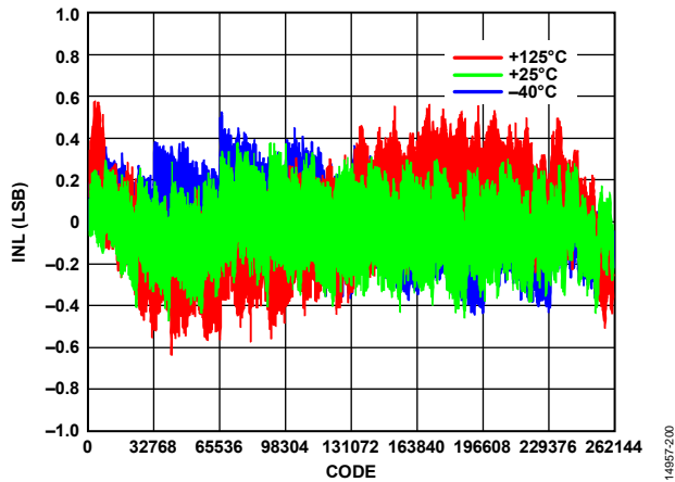
Figure 5. INL vs. Code for Various Temperatures, V_{REF} = 5\text{ V}
