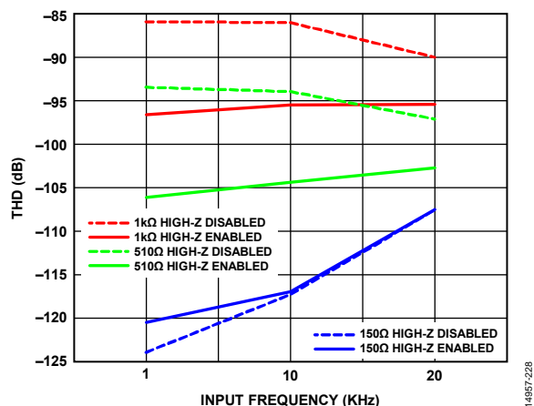
Figure 44. THD vs. Input Frequency for Various Source Impedance, V_{DD} = 1.8 V, V_{IO} = 3.3 V, V_{REF} = 5 V, 25^{\circ}\text{C}
