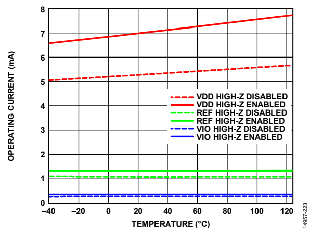
Figure 24. Operating Current vs. Temperature, AD4003, 2 MSPS
