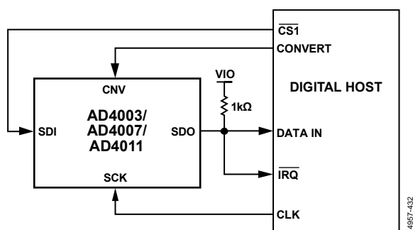
Figure 59. \overline{\text{CS}} Mode, 4-Wire Turbo Mode Connection Diagram
