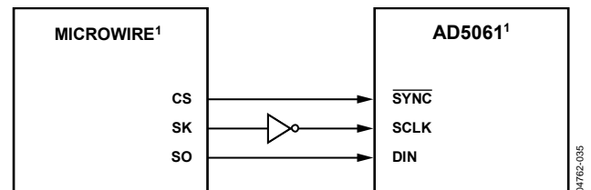
Figure 44. AD5061-to-MICROWIRE Interface
