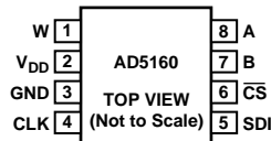
Figure 3. Pin Configuration
