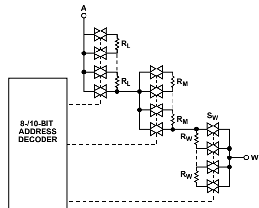
Figure 45. Simplified RDAC Circuit
