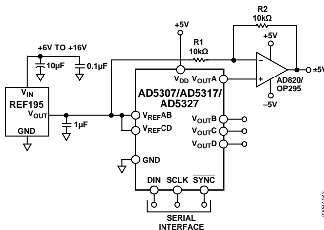
Figure 42. Bipolar Operation with the AD5307/AD5317/AD5327
