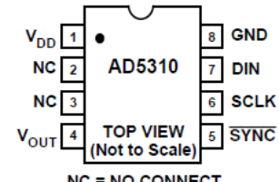
NC = NO CONNECT Figure 4. \mu SOIC
