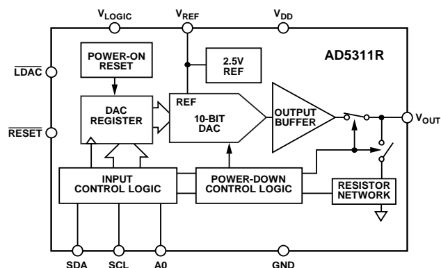
Figure 2. AD5311R
