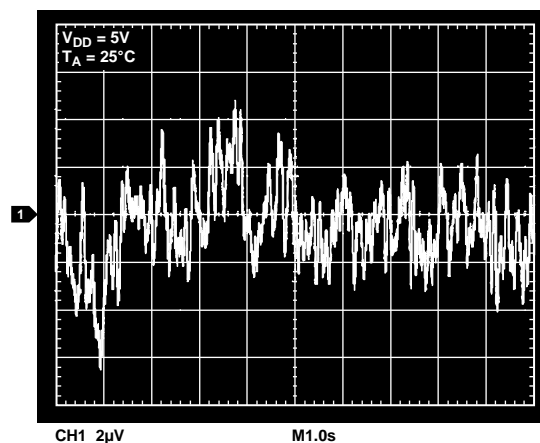
Figure 8. Internal Reference Noise, 0.1 Hz to 10 Hz
