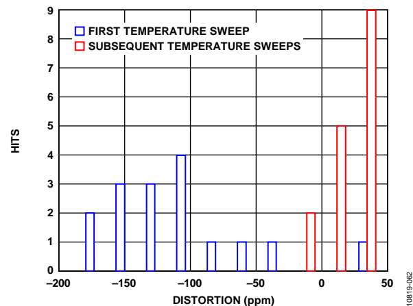
Figure 48. Thermal Hysteresis
