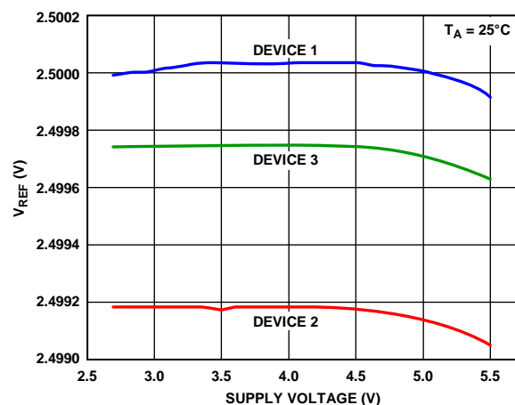
Figure 10. Internal Reference Voltage vs. Supply Voltage
