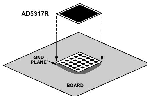
Figure 53. Pad Connection to Board
