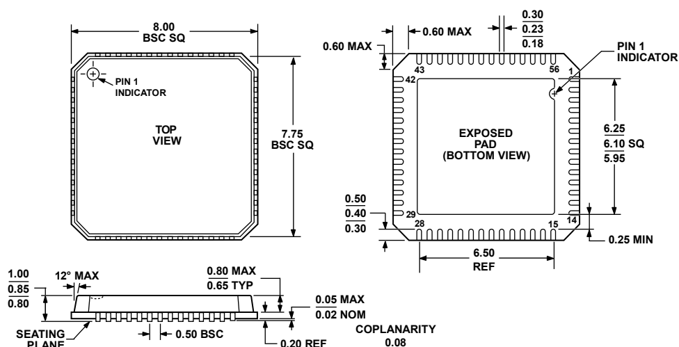
Figure 28. 56-Lead Lead Frame Chip Scale Package [LFCSP_VQ] 8 mm × 8 mm Body, Very Thin Quad (CP-56-1)
