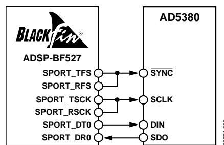
Figure 38. AD5380-to-ADSP-BF527 Interface
