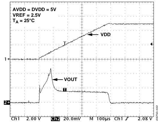
Figure 18. Power-Up Transient
