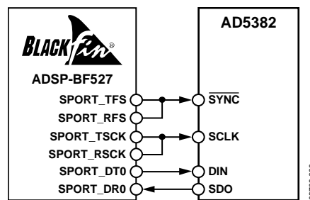
Figure 37. AD5382-to-ADSP-BF527 Interface
