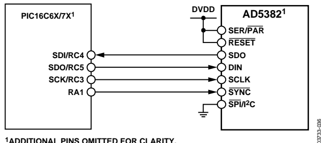
Figure 35. AD5382-to-PIC16C6x/7x Interface
