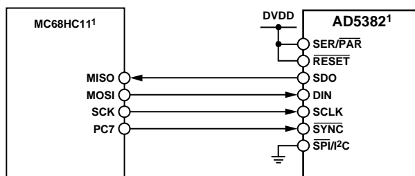
Figure 33. AD5382-to-MC68HC11 Interface
