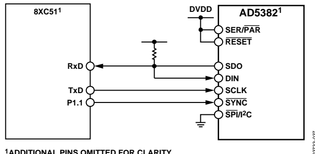
Figure 36. AD5382-to-8051 Interface
