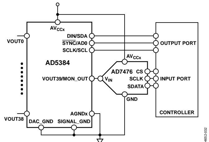
Figure 34. Typical Channel Monitoring Circuit
