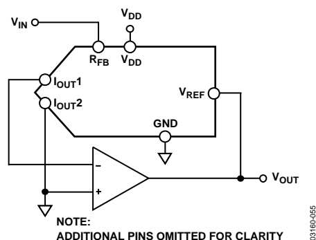
Figure 54. Current-Steering DAC Used as a Divider or Programmable Gain Element
