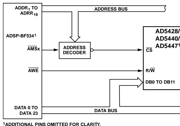
Figure 45. ADSP-BF534-to-AD5428/AD5440/AD5447 Interface
