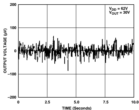
Figure 10. Output Noise
