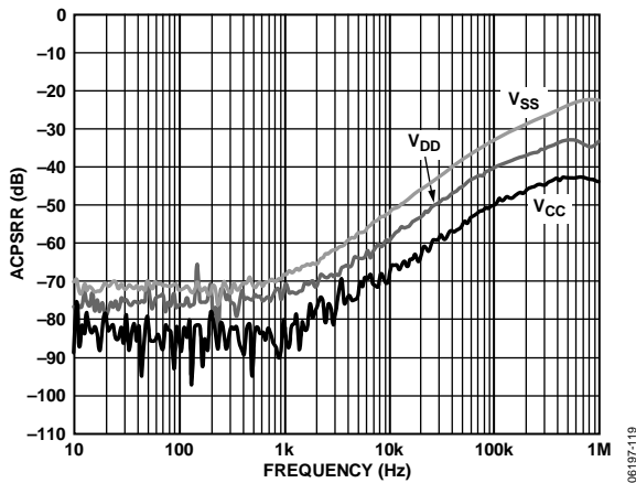
Figure 23. ACPSRR at FOHx in Force Current Mode vs. Frequency (MI Gain = 5)
