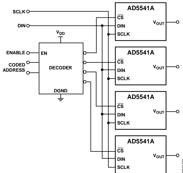
Figure 35. Addressing Multiple DACs
