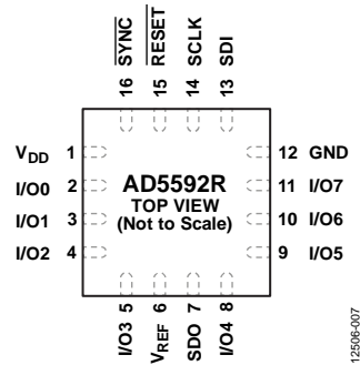
Figure 7. AD5592R 16-Lead LFCSP Pin Configuration
