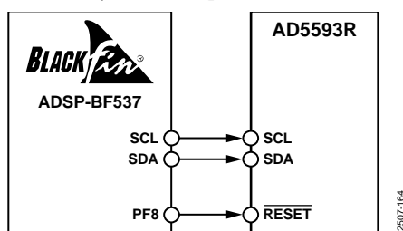
Figure 41. ADSP-BF537 Interface
