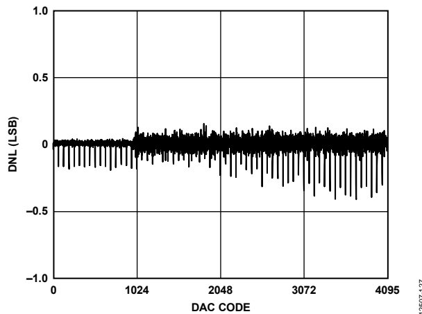
Figure 14. DAC DNL
