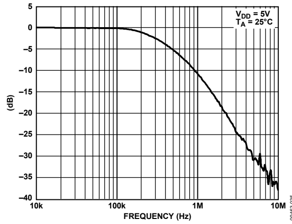
Figure 34. Multiplying Bandwidth
