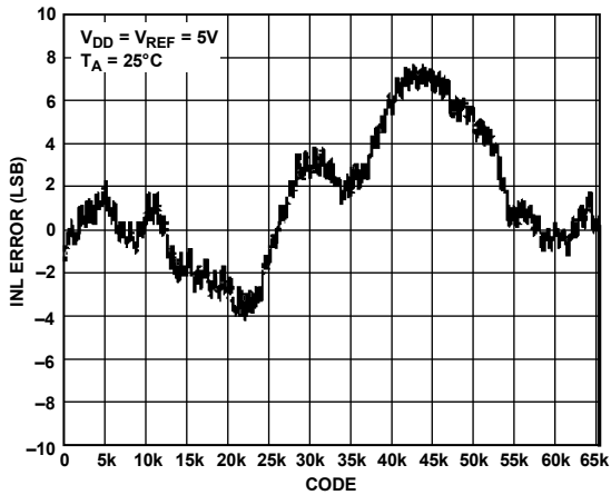
Figure 4. INL—External Reference
