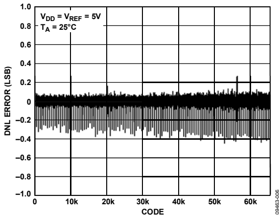
Figure 6. DNL—External Reference
