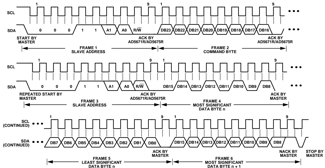
Figure 61. I²C Read Operation
