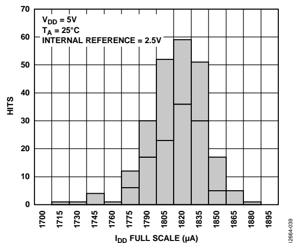
Figure 31. Supply Current ( I_{DD} ) Histogram with Internal Reference
