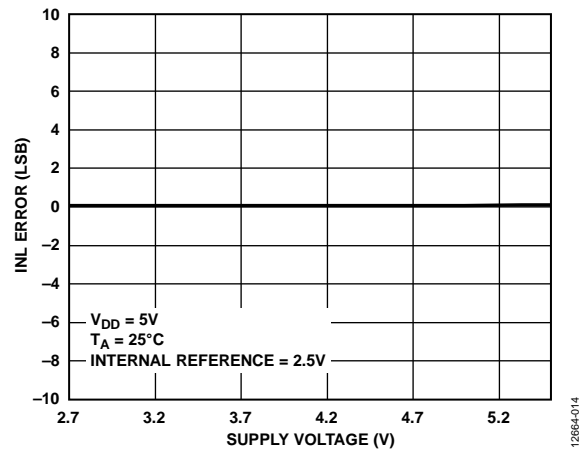
Figure 13. AD5671R INL Error vs. Supply Voltage
