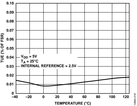
Figure 17. AD5671R TUE vs. Temperature
