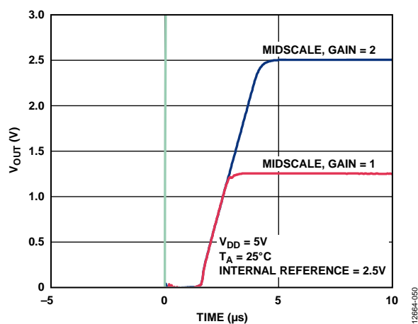
Figure 41. Exiting Power-Down to Midscale
