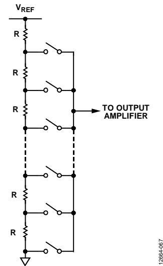
Figure 57. Resistor String Structure
