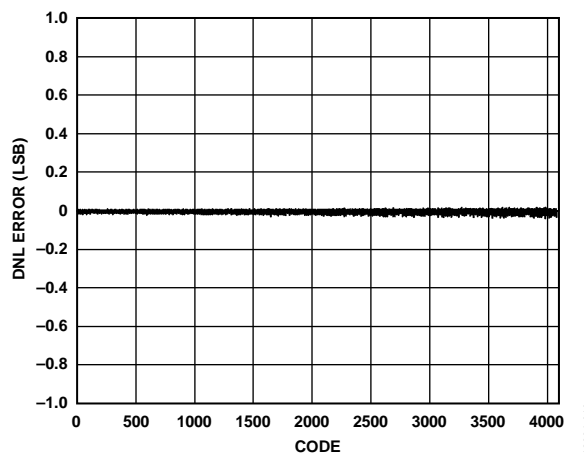
Figure 9. AD5671R DNL Error vs. Code
