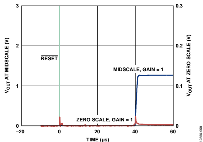
Figure 38. Hardware Reset
