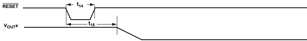
Figure 3. RESET Timing Diagram
