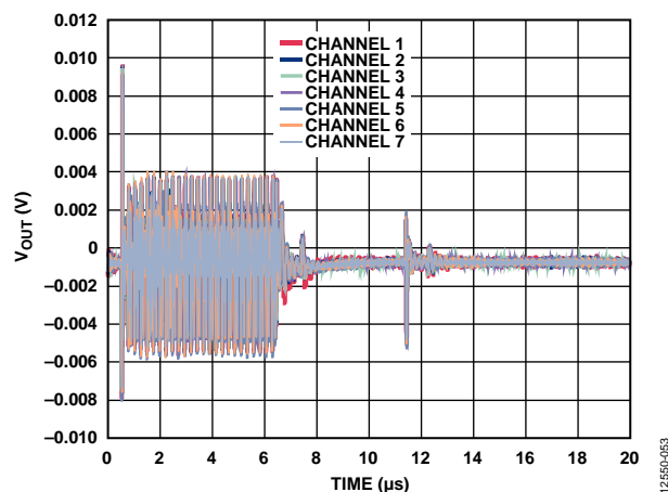
Figure 32. DAC-to-DAC Crosstalk
