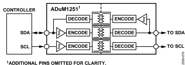
Figure 50. Isolated Interface
