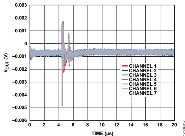
Figure 31. Analog Crosstalk
