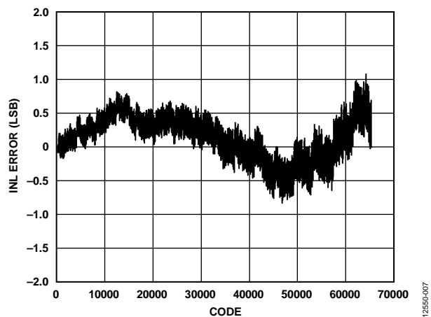
Figure 6. INL Error vs. Code
