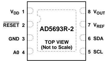
Figure 8. AD5693R-2 Pin Configuration, 8-Lead LFCSP, \overline{\text{RESET}} Option
