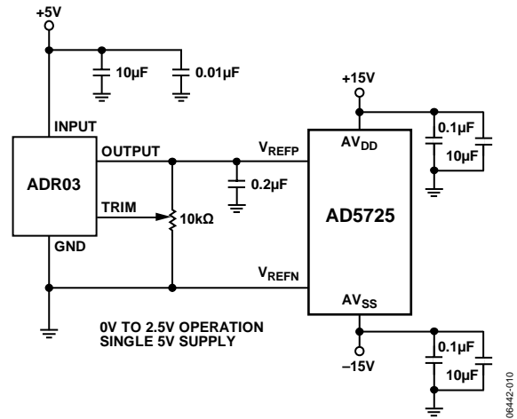
Figure 30. +5 V Single-Supply Operation
