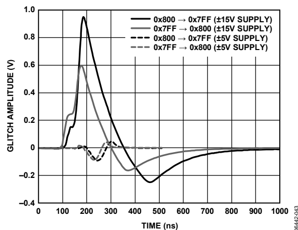
Figure 26. Output Glitch
