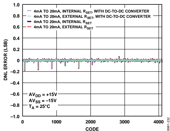
Figure 33. Differential Nonlinearity Error vs. DAC Code
