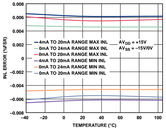
Figure 36. Integral Nonlinearity Error vs. Temperature, External R_{SET}
