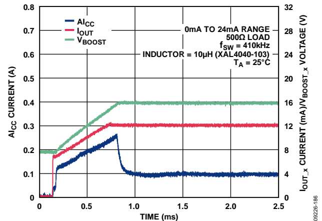
Figure 85. A_{I_{CC}} Current vs. Time for 24 mA Step Through 500 \Omega Load with External 51 k \Omega Compensation Resistor
