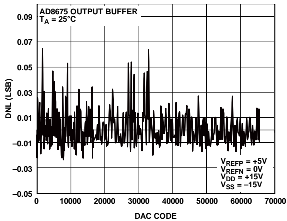
Figure 12. Differential Nonlinearity Error vs. DAC Code, 5 V Span, ×2 Gain Mode
