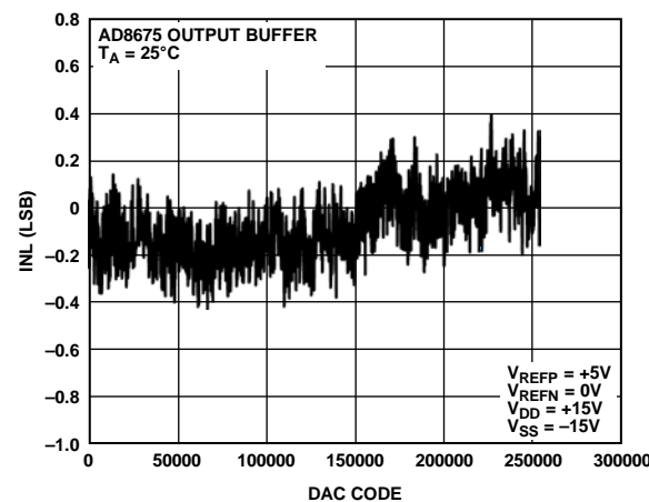
Figure 7. Integral Nonlinearity Error vs. DAC Code, 5\text{ V} Span
