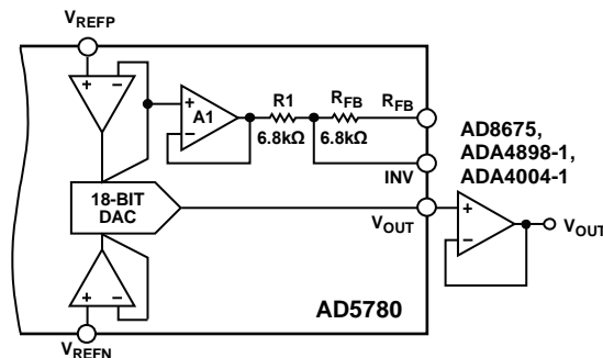
Figure 50. Output Amplifier in Unity-Gain Configuration
