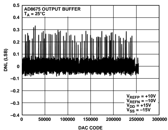
Figure 9. Differential Nonlinearity Error vs. DAC Code, \pm 10\text{ V} Span
