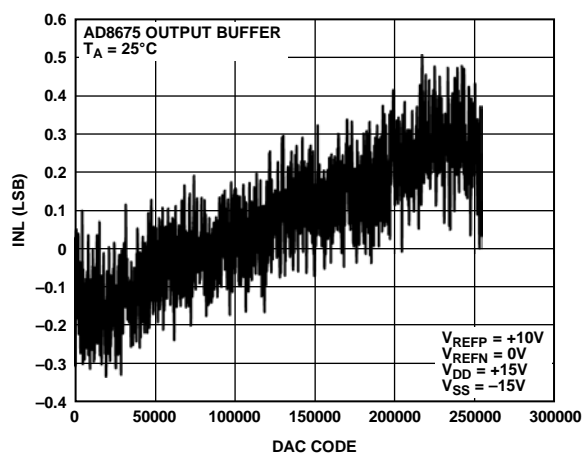
Figure 6. Integral Nonlinearity Error vs. DAC Code, 10\text{ V} Span
