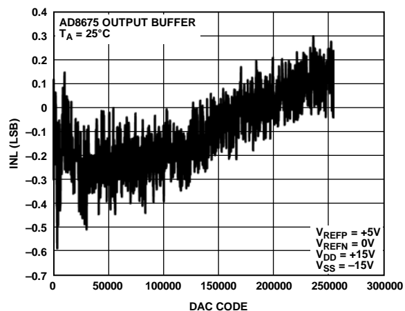
Figure 8. Integral Nonlinearity Error vs. DAC Code, 5\text{ V} Span, \times 2 Gain Mode
