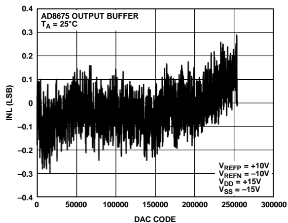
Figure 5. Integral Nonlinearity Error vs. DAC Code, \pm 10\text{ V} Span
