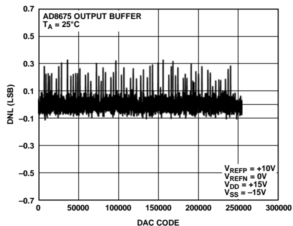
Figure 10. Differential Nonlinearity Error vs. DAC Code, 10\text{ V} Span
