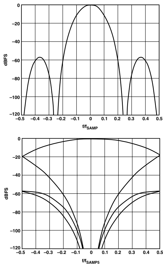
Figure 38. CIC5 Alias Rejection, M_{\text{CIC}5} = 4
