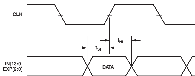
Figure 24. Input Data Timing Requirements
