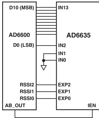
Figure 28. Typical Interconnection of the AD6600 Gain-Ranging ADC and the AD6635.
