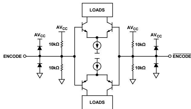
Figure 22. ENCODE/ENCODE-bar Inputs
