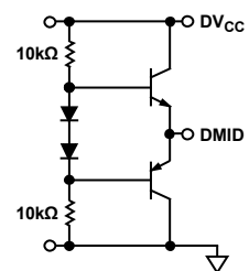
Figure 37. DMID Reference
