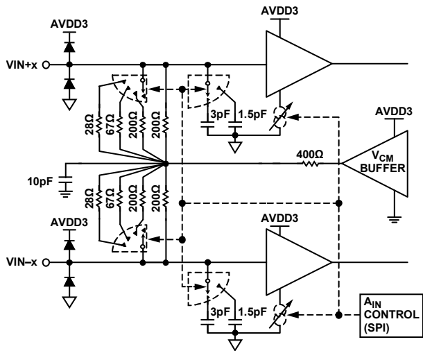
Figure 63. Analog Inputs
