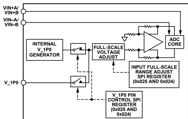
Figure 87. Internal Reference Configuration and Controls
