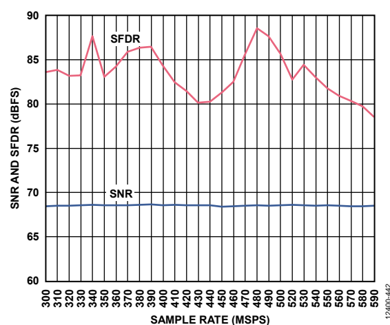
Figure 54. SNR/SFDR vs. Sample Rate ( f_s ), f_{IN} = 170.3 MHz; \text{Buffer Control 1} = 2.0\times
