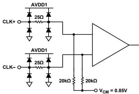
Figure 64. Clock Inputs
