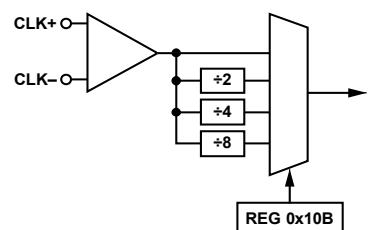
Figure 93. Clock Divider Circuit
