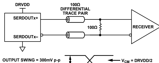
Figure 128. DC-Coupled Digital Output Termination Example
