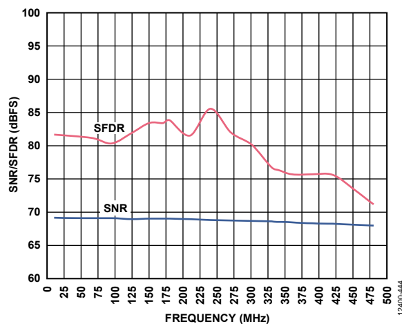
Figure 55. SNR/SFDR vs. Analog Input Frequency ( f_{IN} ); f_{IN} < 500 MHz; \text{Buffer Control 1} = 3.0\times
