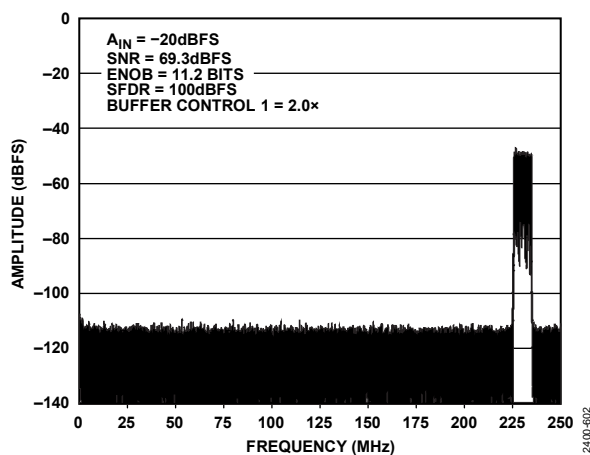
Figure 53. LTE-TDD 10 MHz Channel FFT with f_{IN} = 230 MHz
