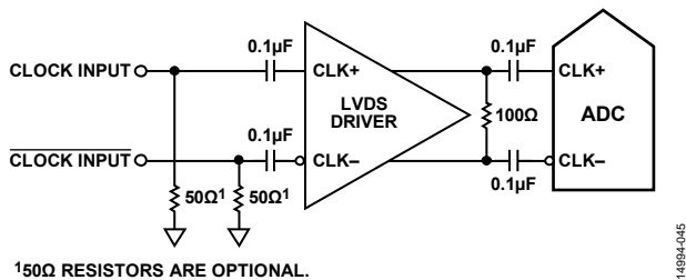
Figure 64. Differential LVDS Sample Clock
