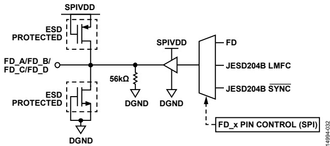
Figure 53. FD_A/FD_B/FD_C/FD_D Outputs
