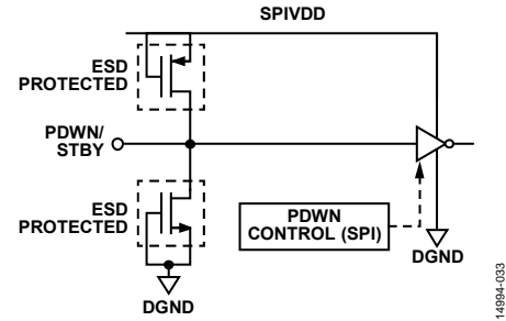
Figure 54. PDWN/STBY Input
