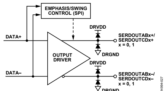
Figure 48. Digital Outputs
