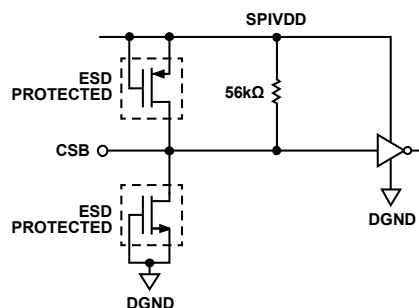
Figure 51. CSB Input
