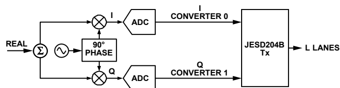
Figure 65. I/Q Transport Layer Mapping
