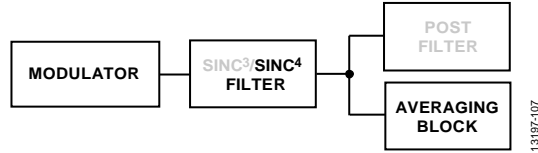
Figure 101. Fast Settling Mode, \text{Sinc}^4 + \text{Sinc}^1 Filter
