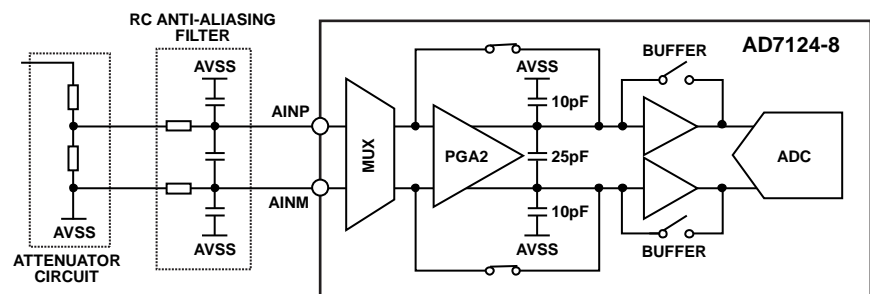
Figure 77. Input Schematic
