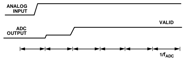
Figure 103. Step Change on the Analog Input, \text{Sinc}^4 + \text{Sinc}^1 Filter
