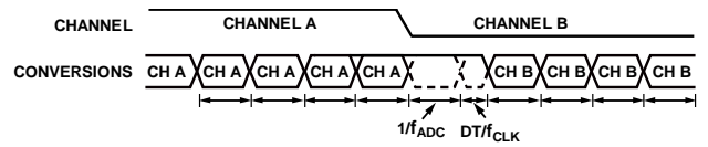
Figure 102. Fast Settling, \text{Sinc}^4 + \text{Sinc}^1 Filter
