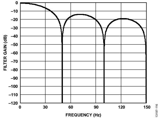
Figure 110. 50 Hz Rejection
