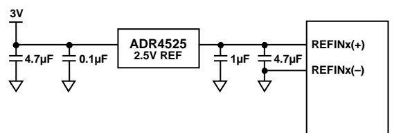
Figure 80. ADR4525 to AD7124-4 Connections
