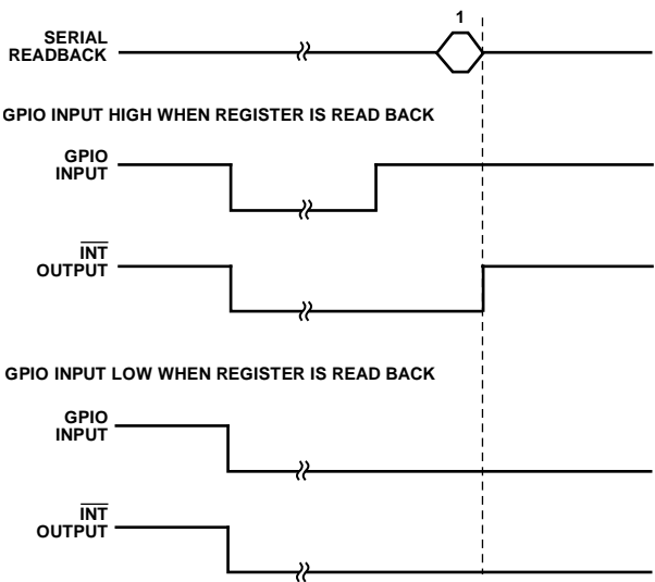
Figure 42. Example of \overline{\text{INT}} Output Controlled by the GPIO Input (GPIO_SETUP = 01, GPIO_INPUT_CONFIG = 00)
