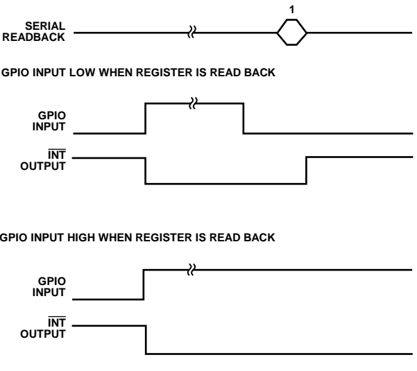
Figure 45. Example of \overline{\text{INT}} Output Controlled by the GPIO Input (GPIO_SETUP = 01, GPIO_INPUT_CONFIG = 11)
