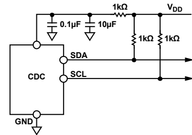
Figure 40. AD7152/AD7153 V_{DD} Decoupling and Filtering
