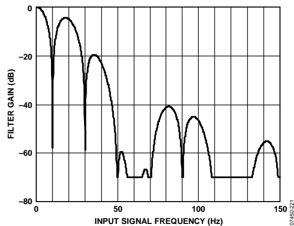
Figure 21. Capacitance Channel Frequency Response, Conversion Time = 50 ms
