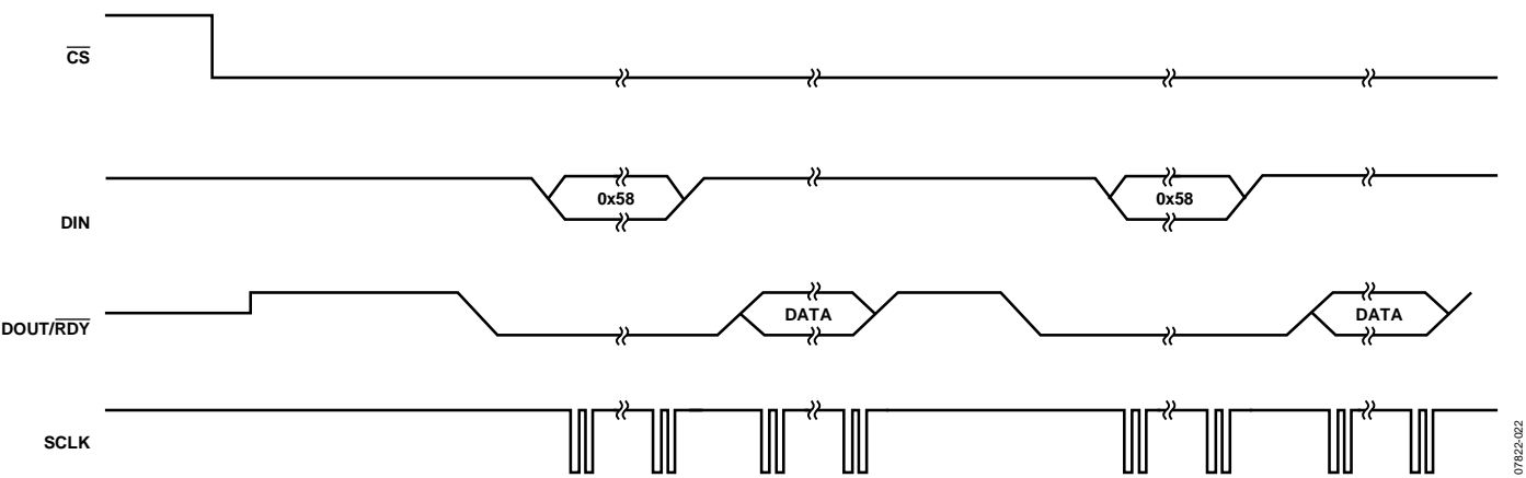
Figure 30. Continuous Conversion
