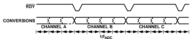
Figure 28. Channel Sequencer
